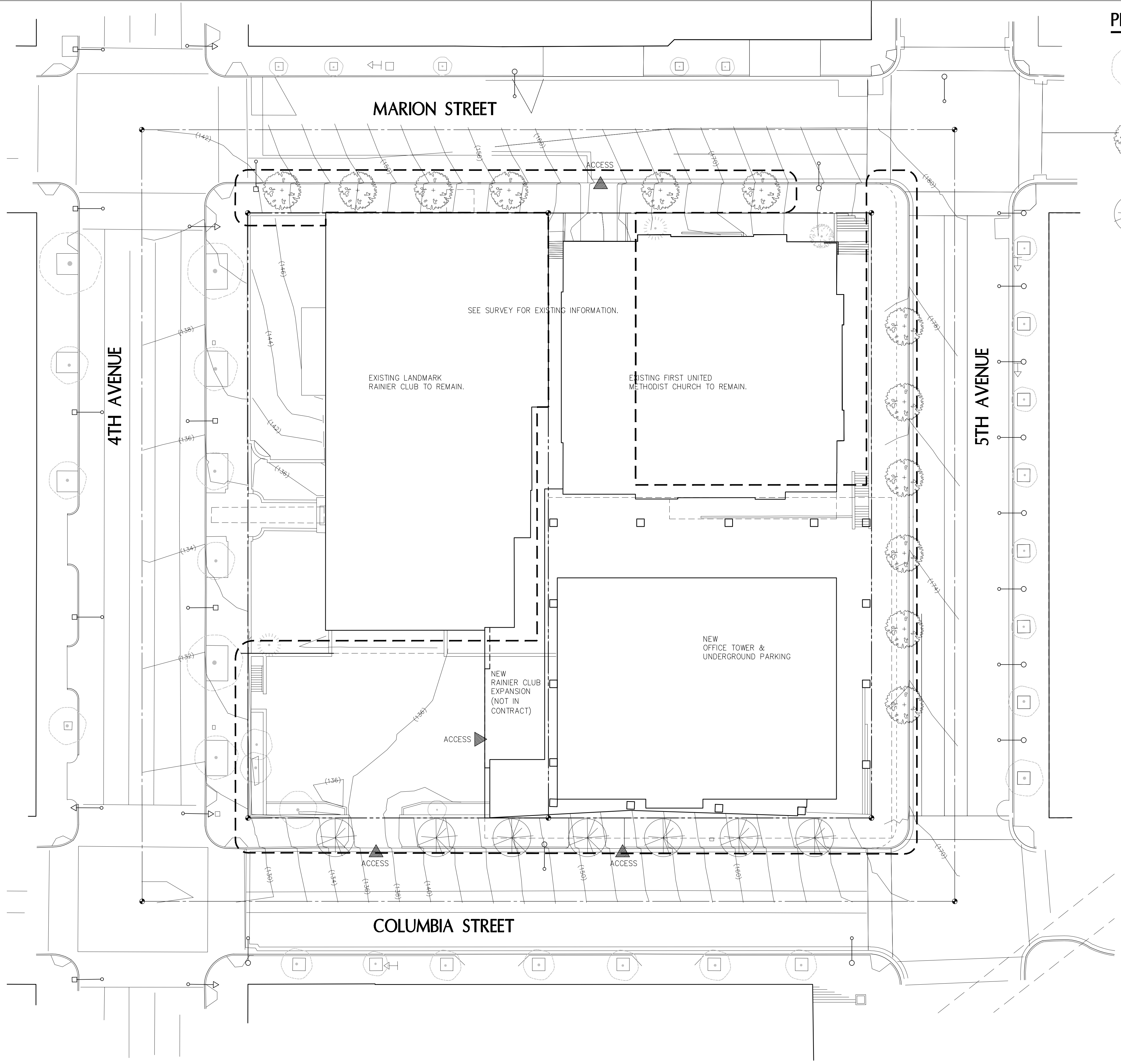
1 STREET TREE PLAN L3-00 SCALE: 1" = 20'
