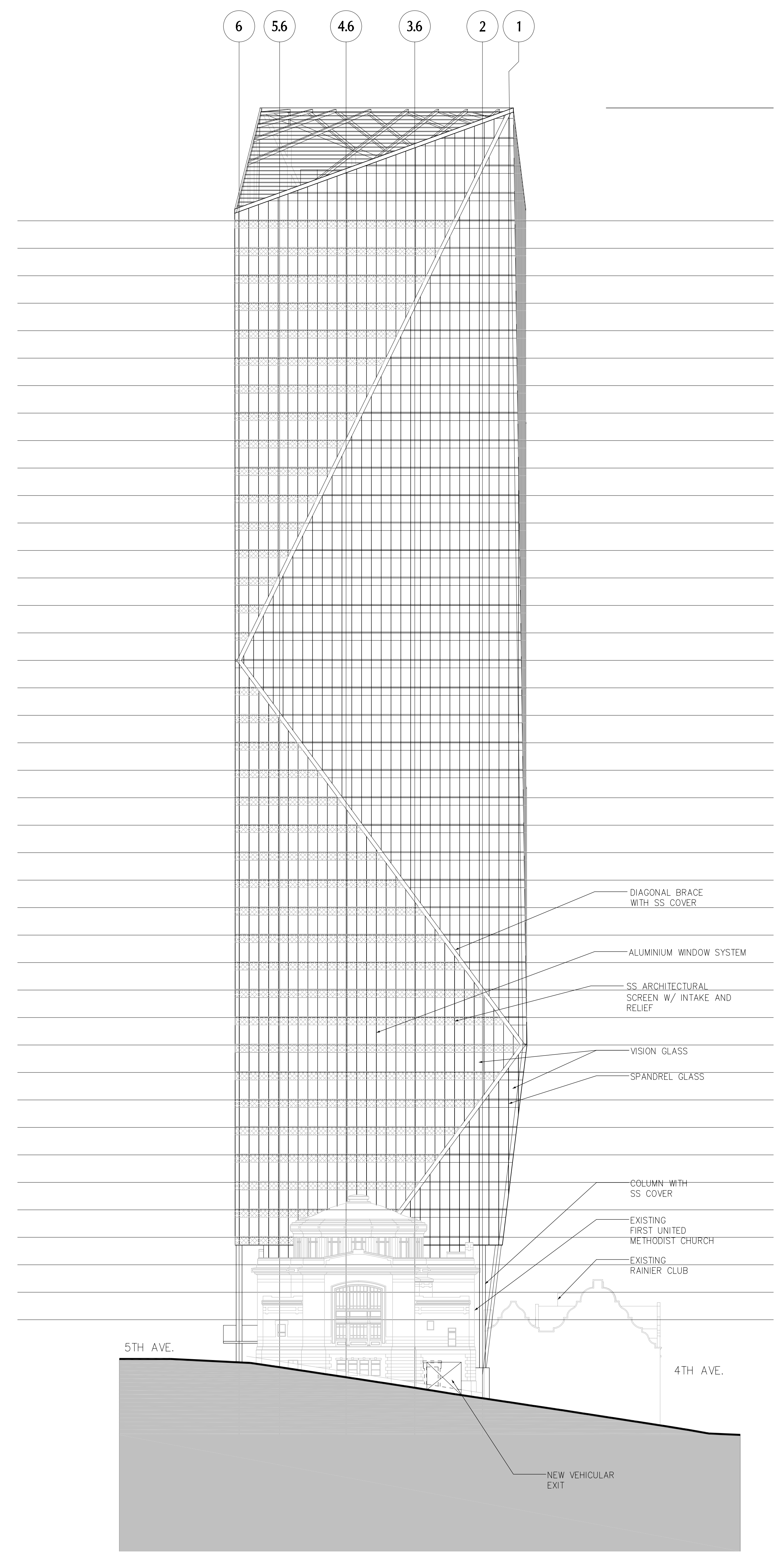
1 ELEVATION - NORTH (MARION STREET) A3.02 SCALE: 1" = 30'
