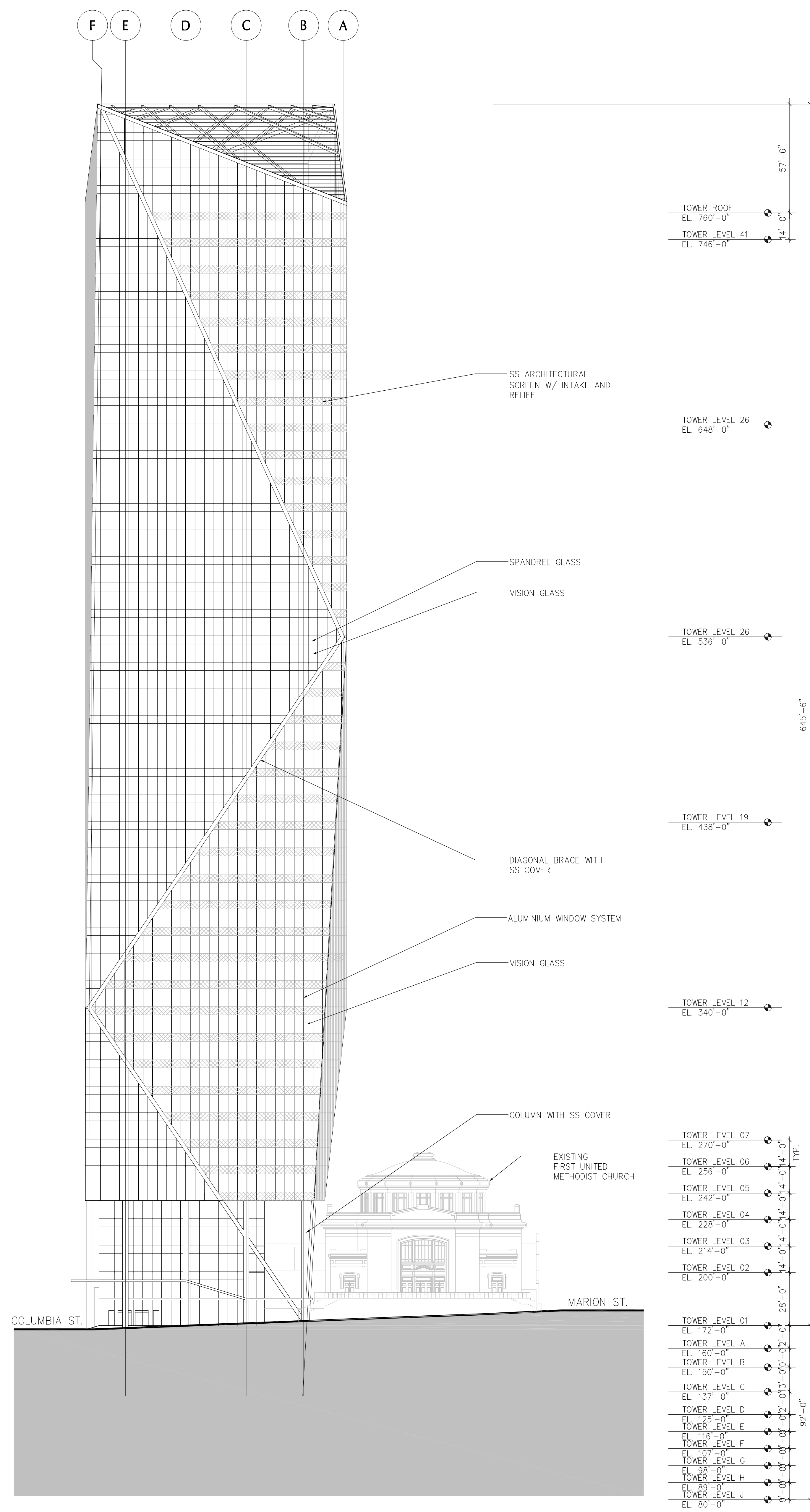
1 ELEVATION - EAST (5TH AVENUE) A3.01 SCALE: 1" = 30'
